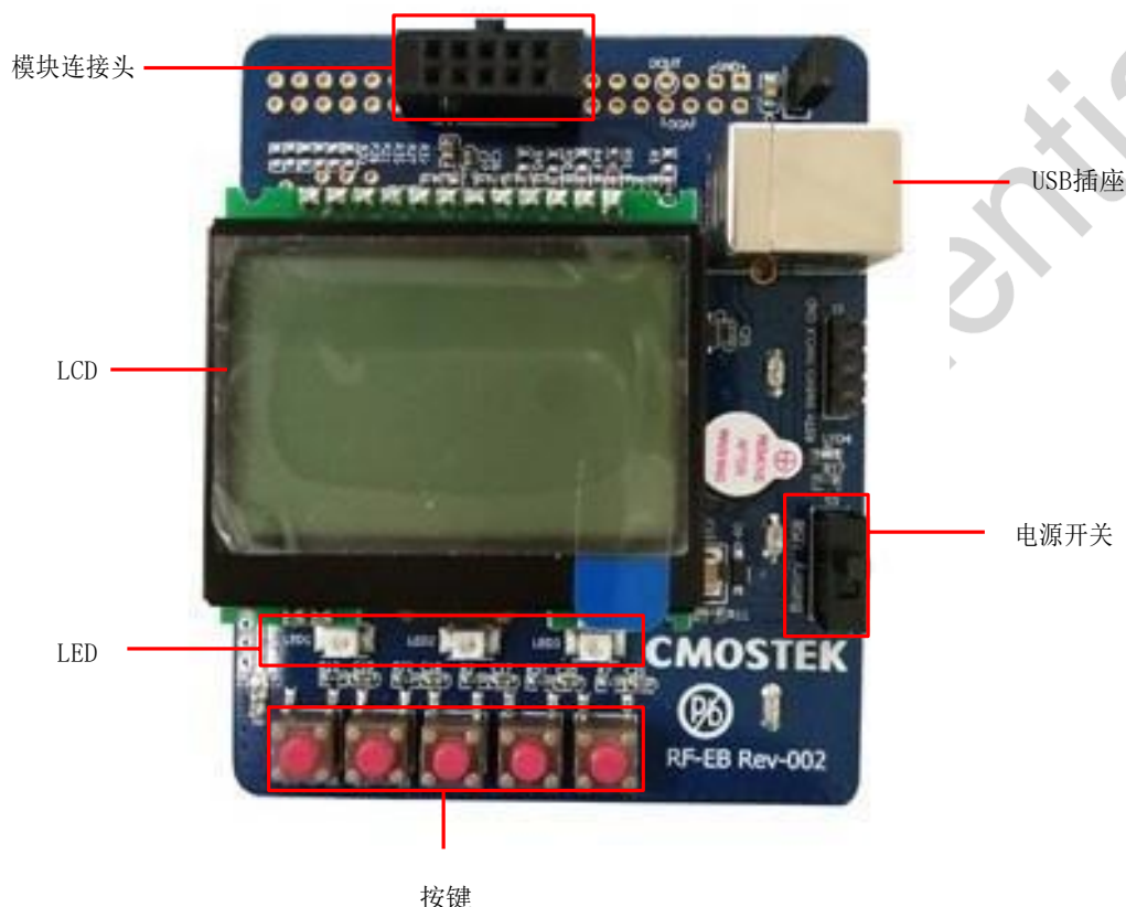
Figure1. Evaluation Motherboard
